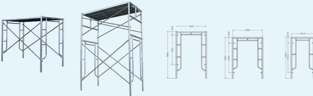
Frame scaffolding -Type 1
