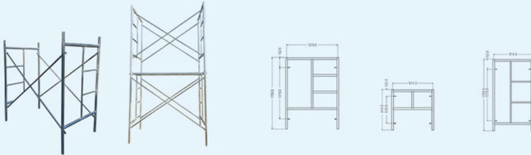
Frame scaffolding -Type 2
